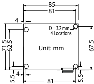
Local/Remote Extender Dimensions
